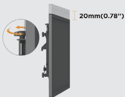
Height Adjustment
